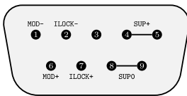
SubD-9 male
