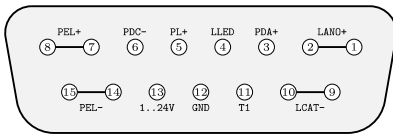
SubD-15 female
